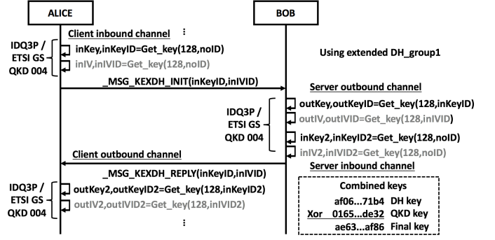
Fig. 3. Diffie-Hellman and QKD key exchange protocol integration.
